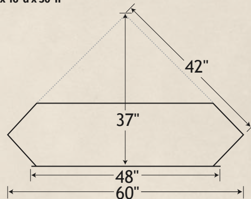
6030C 60" Corner TV Console 60"w x 16"d x 30"h
